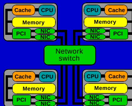
Channel bonding in a cluster
