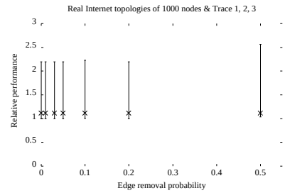
Fig. 10. A summary of the relative performance of the greedy algorithm during edge removal using errorbars. The lower and upper bounds, and the X mark on each errorbar correspond to the minimum, maximum, and median, respectively, of the relative performance of the greedy algorithm.
