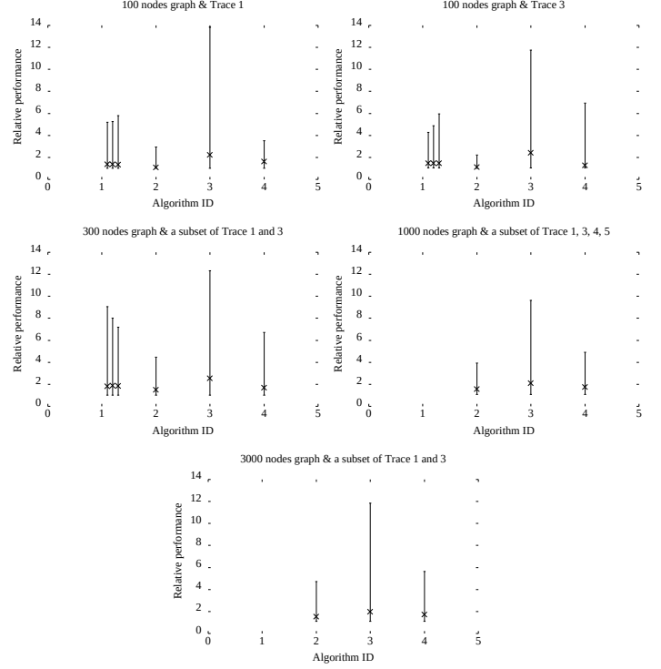
Fig. 5. A summary of the performance of the placement algorithms on graph topologies using errorbars. The lower and upper bounds, and the X mark on each errorbar correspond to the minimum, maximum, and median, respectively, of the relative performance of the corresponding algorithm. The tree-based, greedy, random, and hot spot algorithms are respectively numbered 1, 2, 3, and 4 in the graph.
