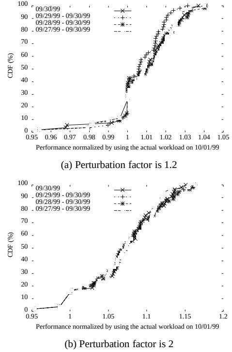
Fig. 12. The CDF of the greedy algorithm’s performance using the predicted workload normalized by its performance using the actual workload when we also perturb the distance between any two nodes.
