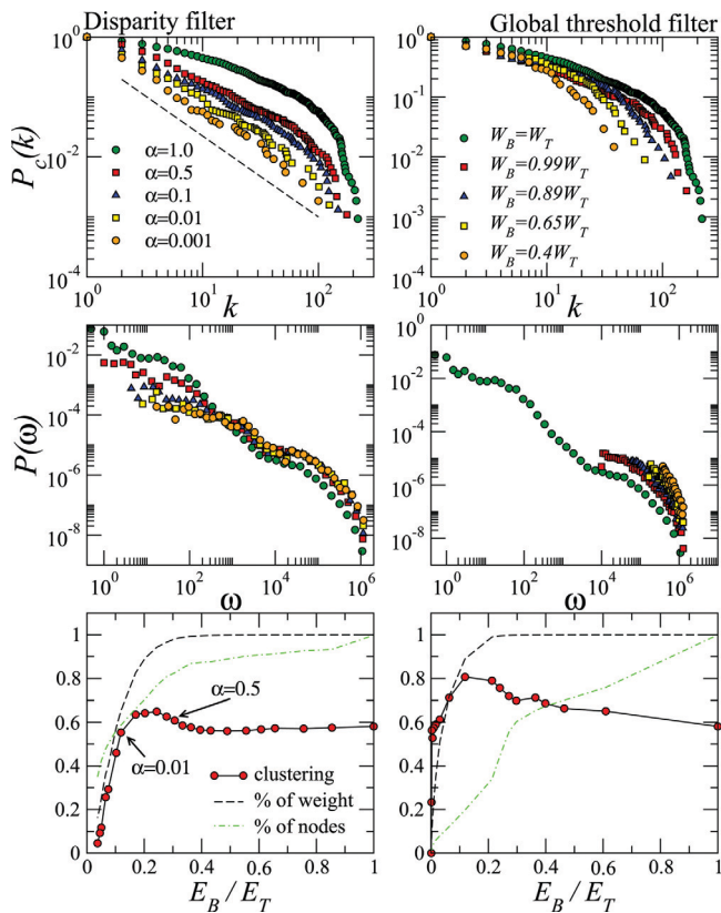
Fig. 2. Topology of the filtered subgraphs for the U.S. airports network. ( Top ) Cumulative degree distribution, P_c(k) , for the disparity ( Left ) and global threshold ( Right ) backbones. The values of \omega_c on the right plot are chosen to generate subgraphs with the same weight as the ones shown on the left plot. ( Middle ) Distribution of links' weights of the different subgraphs generated by the two filters. Symbols are the same as in the top plots. ( Bottom ) Clustering coefficient averaged over nodes of degrees >1 for the two methods as a function of the fraction of edges in the backbones. Dashed lines show the fraction of nodes and weight for a given fraction of edges.
