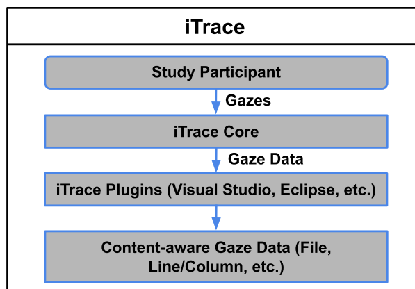
Fig. 2. The architecture of iTrace
