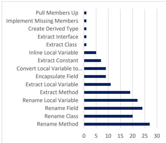
Fig. 6. Types of refactorings that participants most want to see automated. Participants were allowed to select more than one. Additionally, developers were allowed to write in refactorings they wanted to see automated but that were not listed in the question. These were added to this figure.
