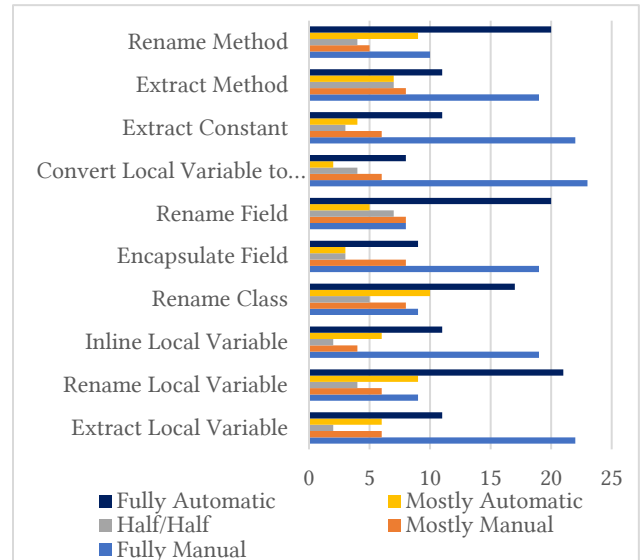
Fig. 7. Frequency at which participants currently automatically or manually apply common refactorings.
