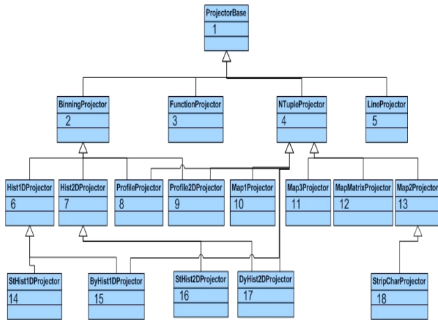
Figure 7. A Partial UML Class-diagram for Projectors - Multiple-Inheritance
