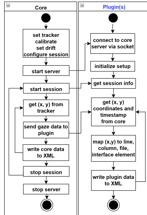
Figure 1: Overview of the iTrace architecture
