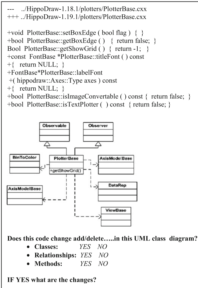
Fig. 10 One of the 24 test problems given to human experts. The line differences are the relevant output of the diff utility. The UML class diagram is the pertinent parts of the system before the design change. Based on this information, the expert answered the questions at the bottom regarding changes to the design
