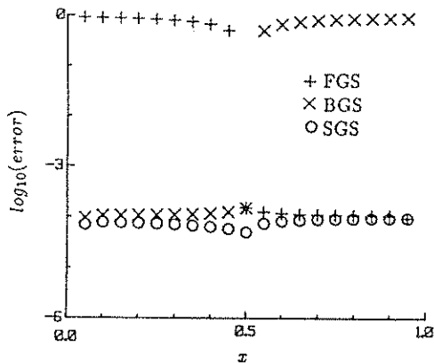
Figure 3: Log of error after first iteration for problem (17)
