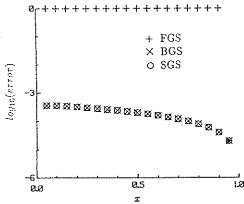
Figure 1: Log of error after first iteration for problem (8)
