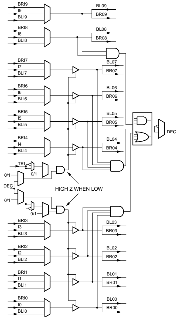
Figure 2. SLIC All Modes Diagram
