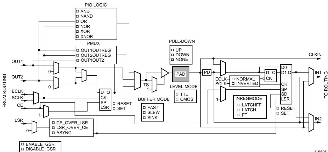
Figure 3. OR3Cxx Programmable Input/Output (PIO) Image from ORCA Foundry
