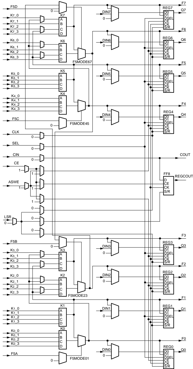
Figure 1. Simplified PFU Diagram
