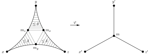
Figure 2: A geodesic triangle \Delta(x, y, z) , the points m_x, m_y, m_z , and the tripod \Upsilon(x', y', z') .
