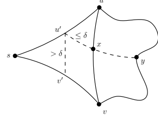
Figure 4: To the proof of Proposition 8: if d_G(u', v') > \delta , then d_G(s, y) < d_G(s, u) .
