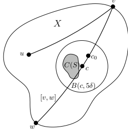
Figure 3: Computing \{v, w\} and c via two FP scans.
