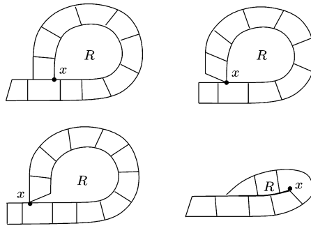
Fig. 1. To the proof of Lemma 4.2.
