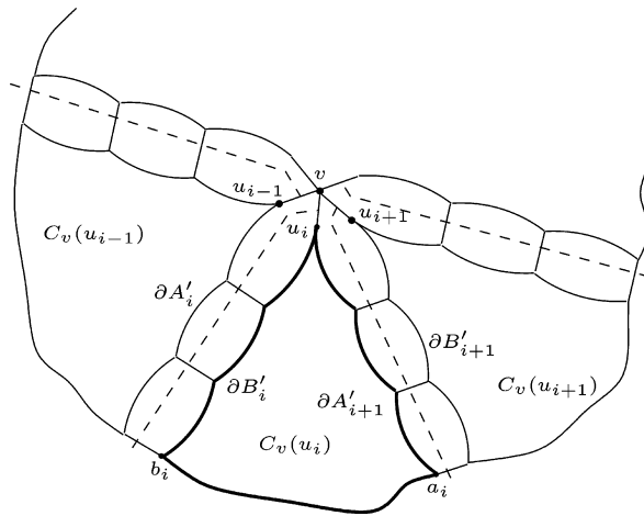
Fig. 4. The cone C_v(u_i) .
