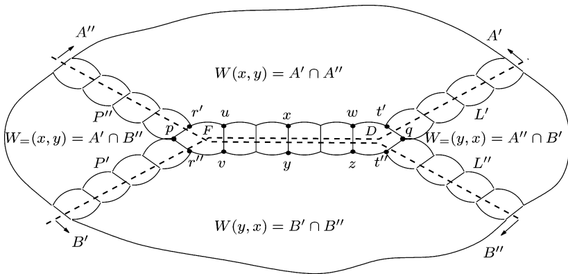
Fig. 3. The relationship between A', B', A'', B'' and W(x, y), W(y, x), W_=(x, y) .
