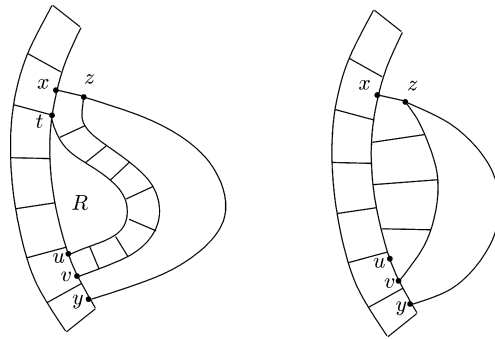
Fig. 2. To the proof of Lemma 4.3.
